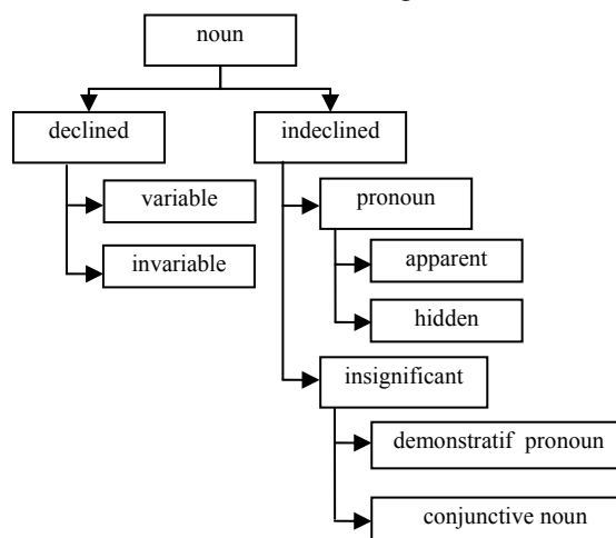
Figure 2. Noun's categories
