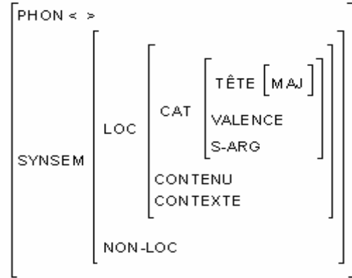
Figure 6. The Structure of an AVM
