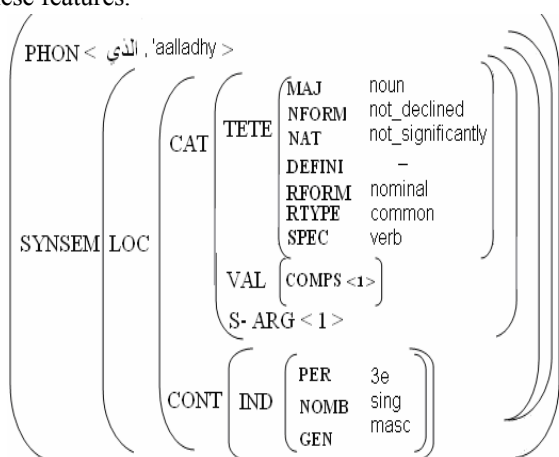
Figure 8. The Arabic relative pronoun features
