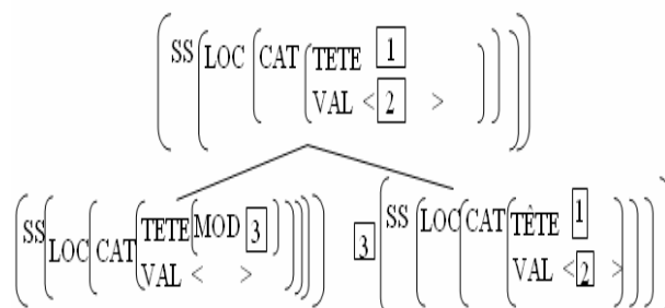
Figure 10. The rule of modification: modified schema
