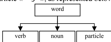
Figure 1. Arabic word
