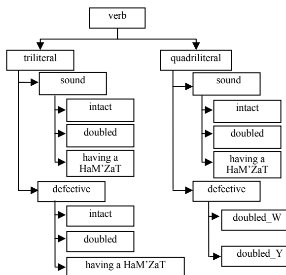
Figure 3. Verb's categories
